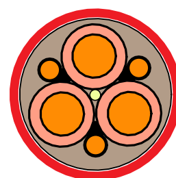
Fig. 9 Medium voltage pump cable
