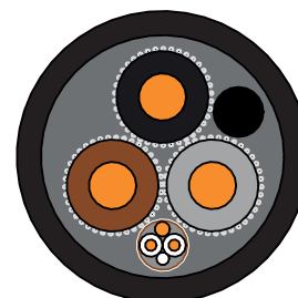
Fig. 3 Screened SUBCAB® - 1.5 mm 2
