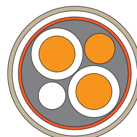
Fig. 6 SUBCAB® - control element design in fig. 1,2,3 and 5
