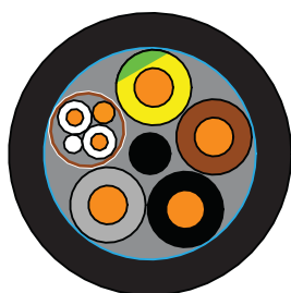
Fig. 1 SUBCAB® - 10-35 mm 2
